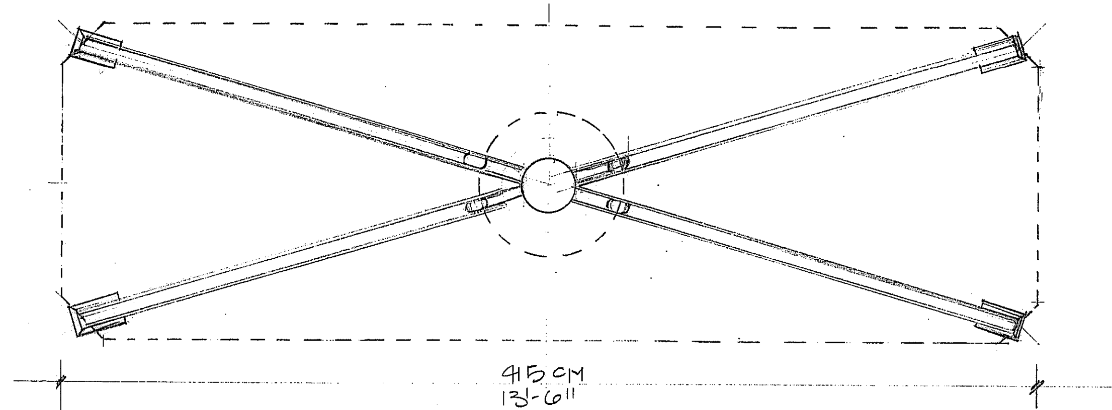
PLAN - BASE
